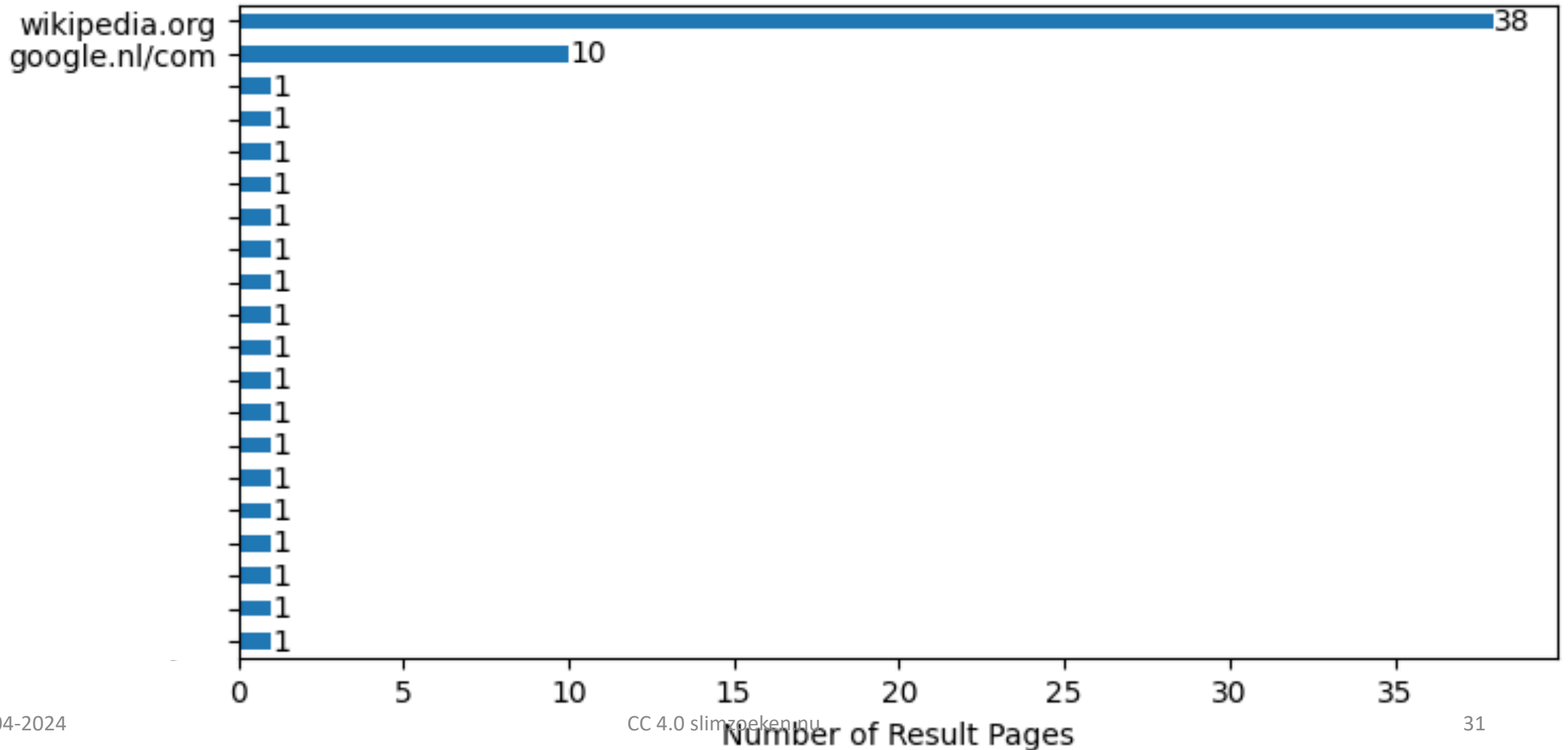
20 most common Sources across Top 1 Search Results (out of 100)
